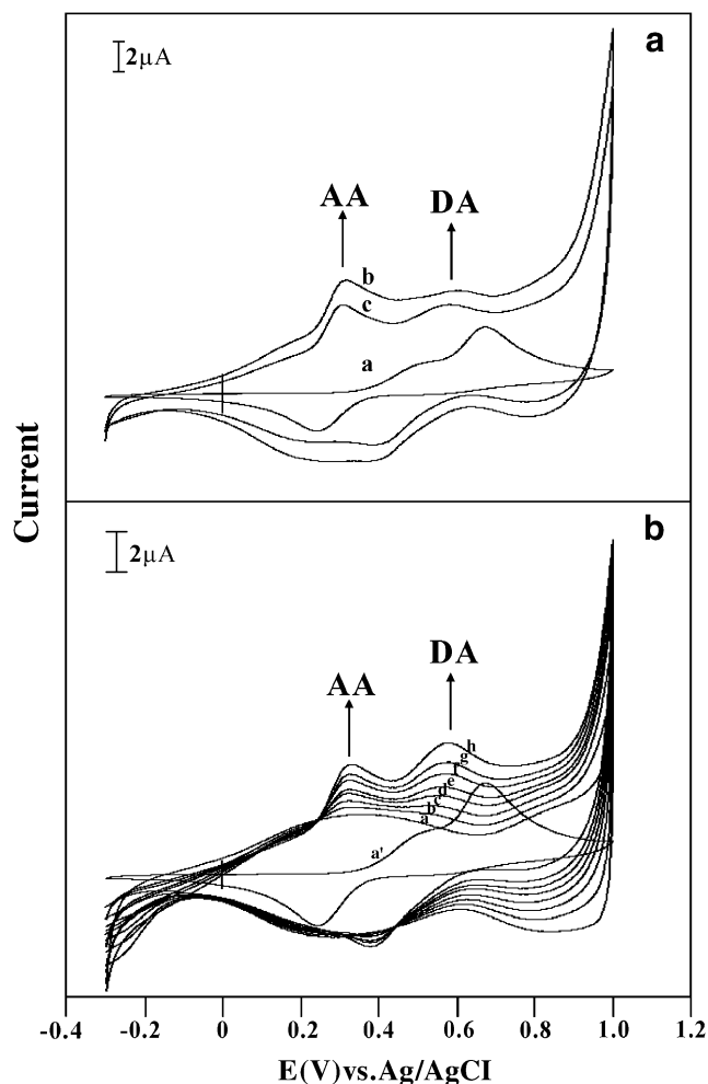
Fig. 7 a CVs were recorded in 0.1 M \text{KNO}_3 solution containing 400 \mu\text{M} [DA] and 400 \mu\text{M} [AA] using (a) bare GC electrode, (b) RuOx–Nf, and (c) RuOx-modified electrodes. b Simultaneous measurements of DA and AA at RuOx–Nf–GC, [DA] = [AA] = (a) 0.0, (b) 50, (c) 100, (d) 150, (e) 200, (f) 250, (g) 300, (h) 350, and (a') bare GC with [DA] = [AA] = 350 \mu\text{M}
