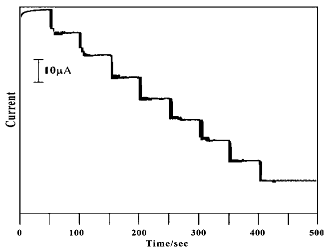
Fig. 9 Amperometric current-time curves for eight successive addition of 50 μM DA into 0.1 M KNO 3 at RuO x -Nf-GC-film-modified electrode. Electrode rotation speed ~600 rpm and applied potential +600 mV (vs. Ag/AgCl)
