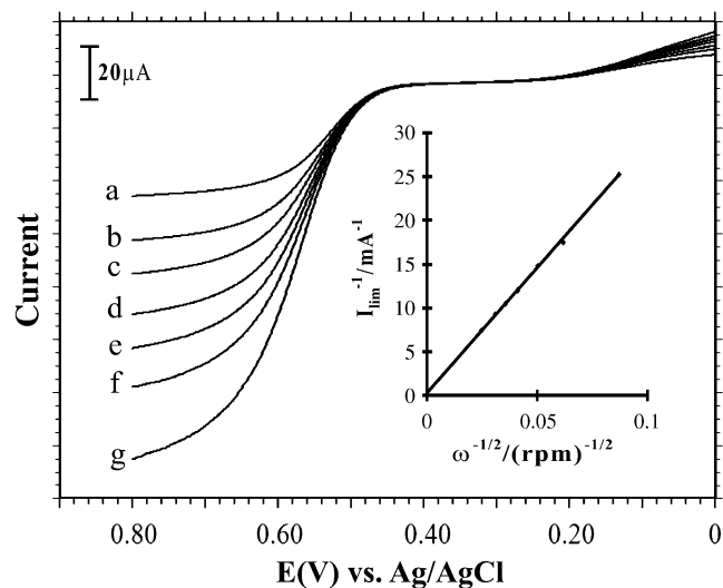
Fig. 10 RDE voltammograms of RuO x -Nf film adsorbed on a GC disk electrode in an aqueous 0.1 M KNO 3 solution with [DA] 350 μM and rotation rate (a) 200, (b) 400, (c) 600, (d) 900, (e) 1,200, (f) 1,600, and (g) 2500 rpm. Scan rate=0.015 V/s. Inset figure shows plots of I_{lim}^{-1} vs. \omega^{-1/2}
